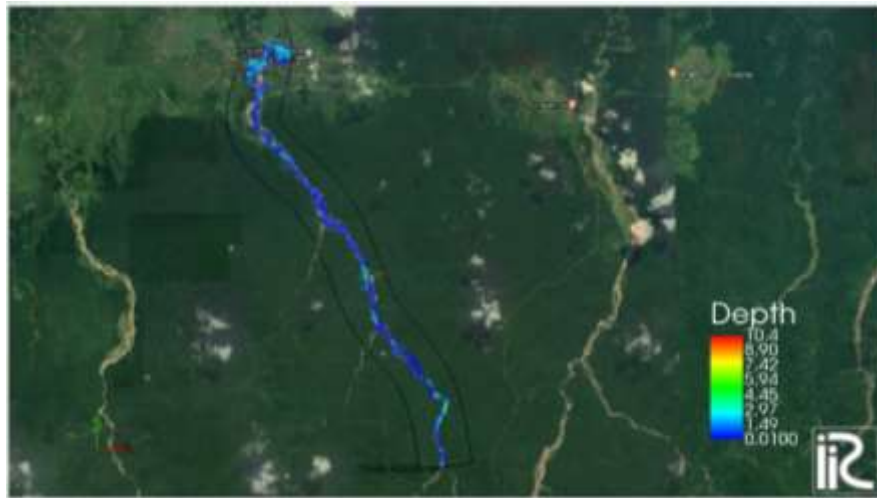
Figure 6. Visualization of iRIC software simulation results
