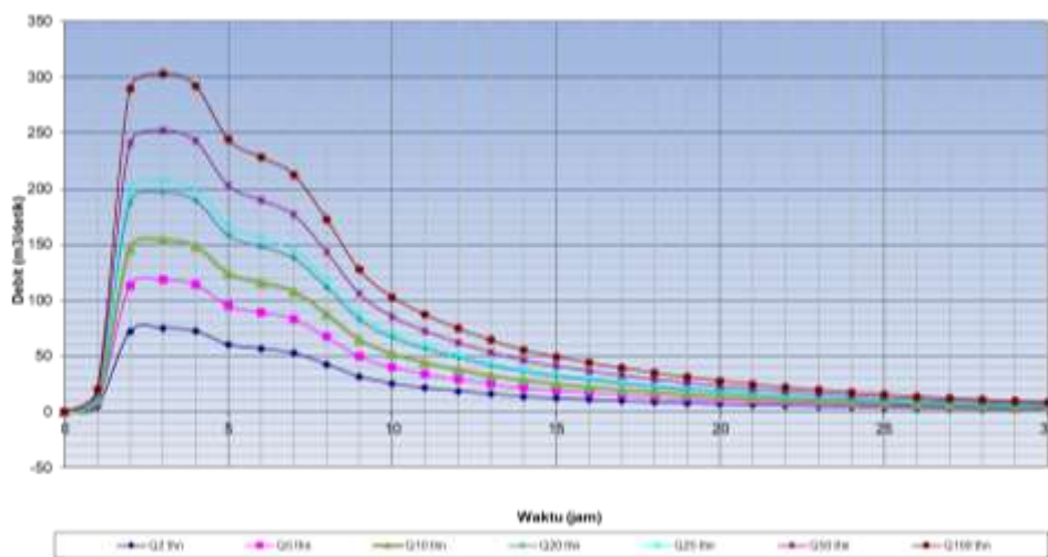
Figure 7. Discharge plan for Nakayasu HSS method
