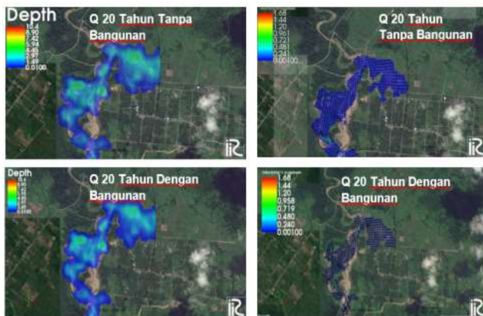
Figure 10. Simulation of depth and speed with Q20 years
